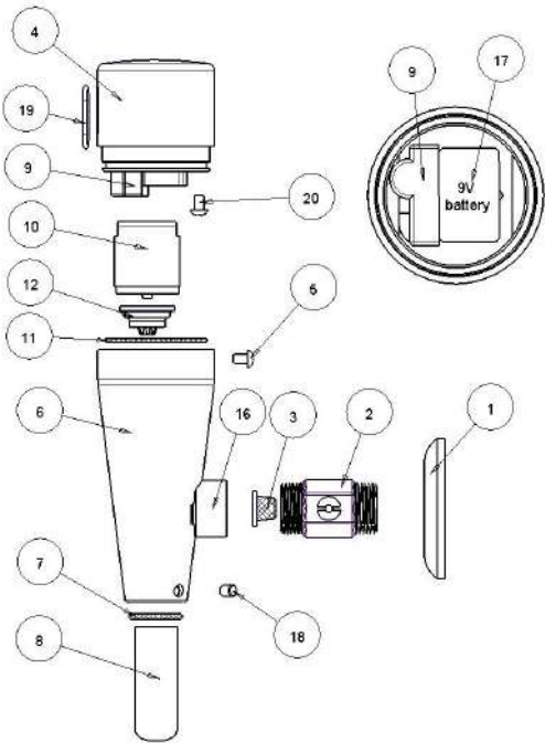
Explosed electronic flush valve - Free
